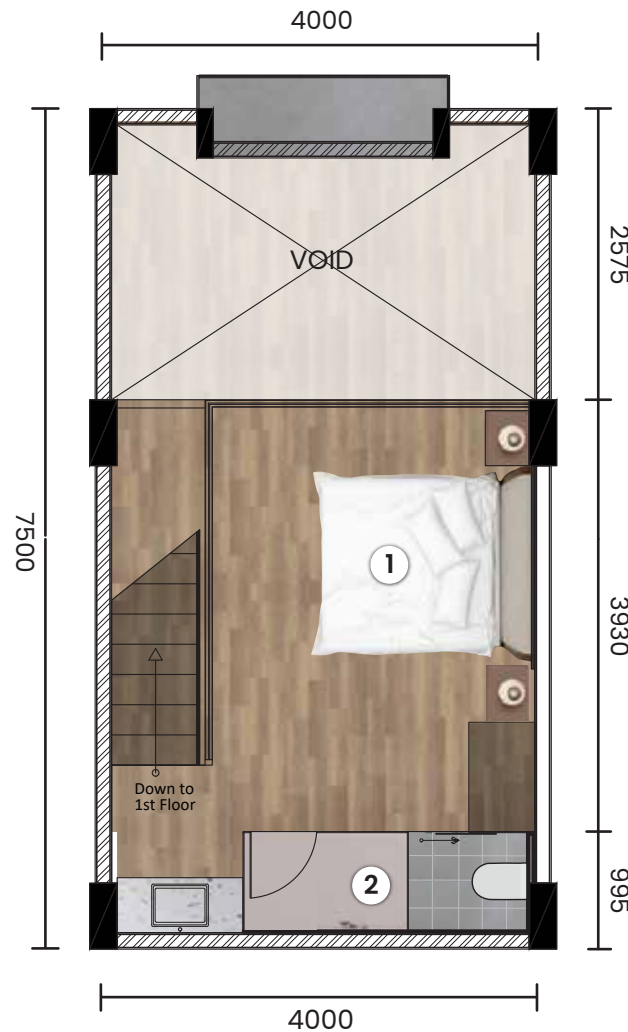
MEZZANINE PLAN
